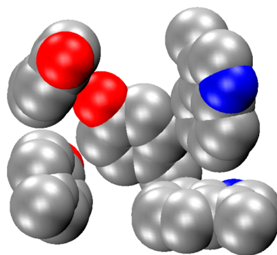
FIGURE 3. The aromatic box from AChBP (pdb file 119B).
